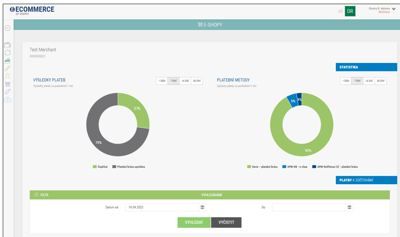
Obr. 23: Nabídka E-shopy
